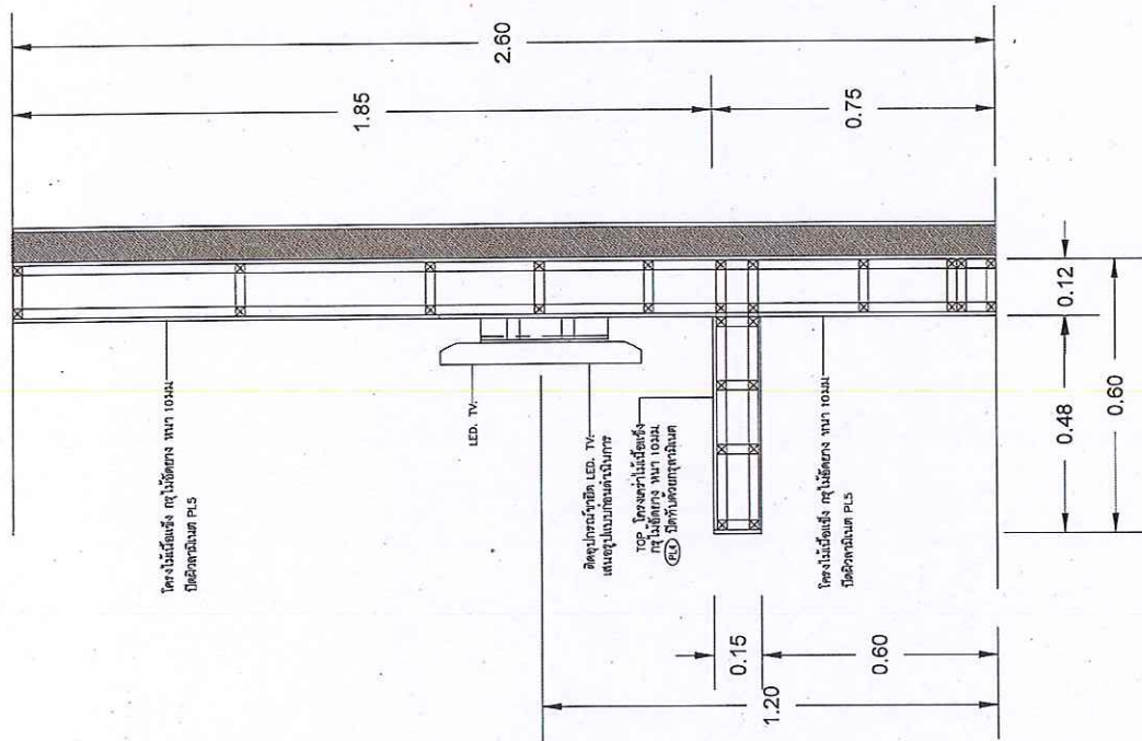
B:02/1 SECTION 1
