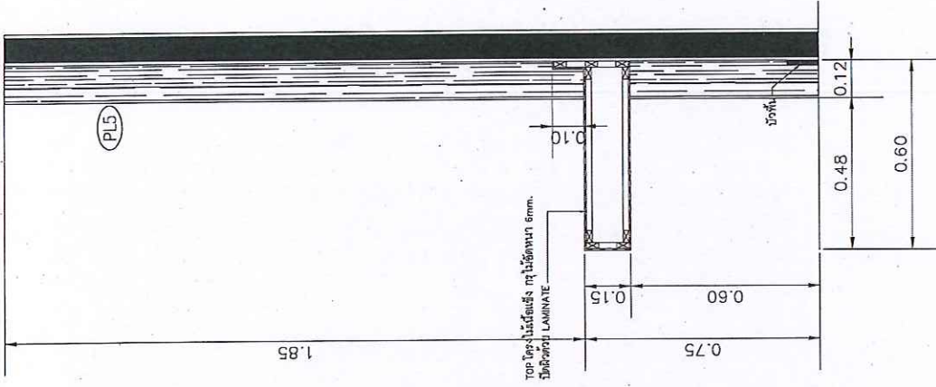
B:02/1 SECTION 2
